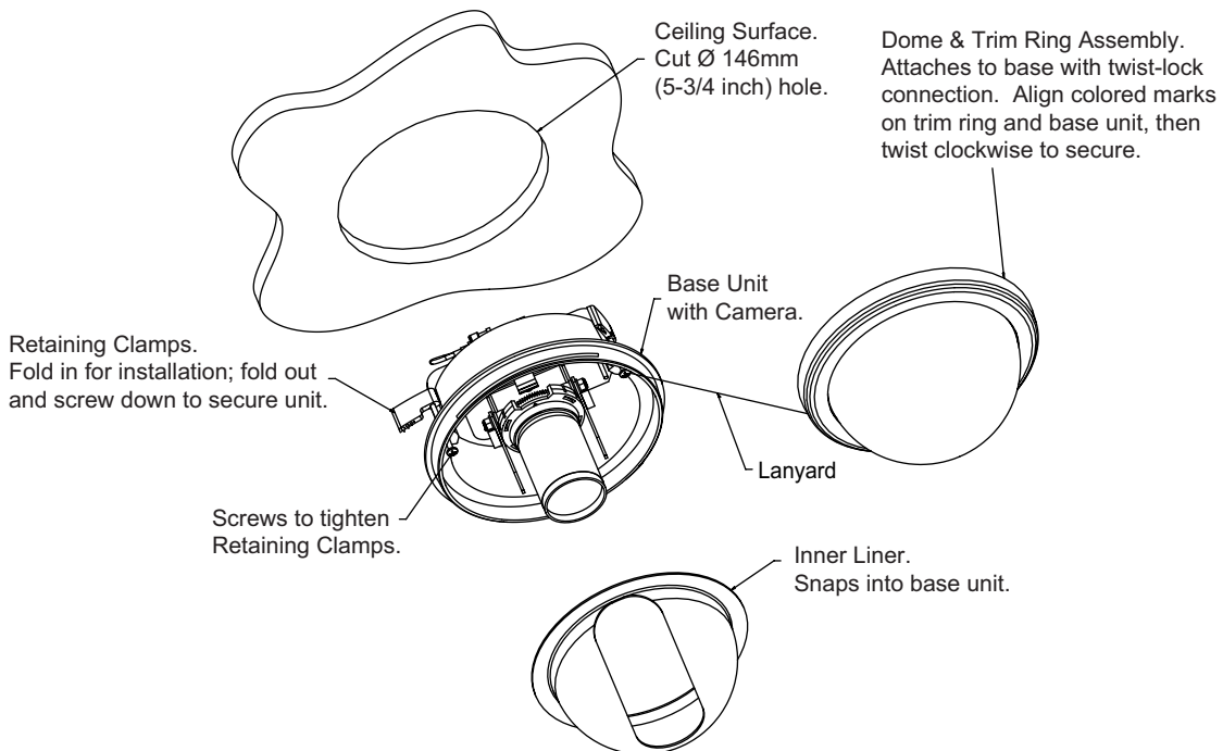
Figure 2 In-ceiling Installation
